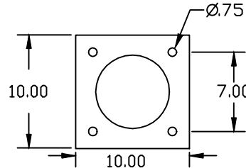
PLAN VIEW - BASE PLATE (Used On Carbon Steel Bollard)
