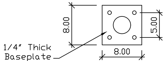
PLAN VIEW - BASE PLATE (Used On Carbon Steel Bollard)
