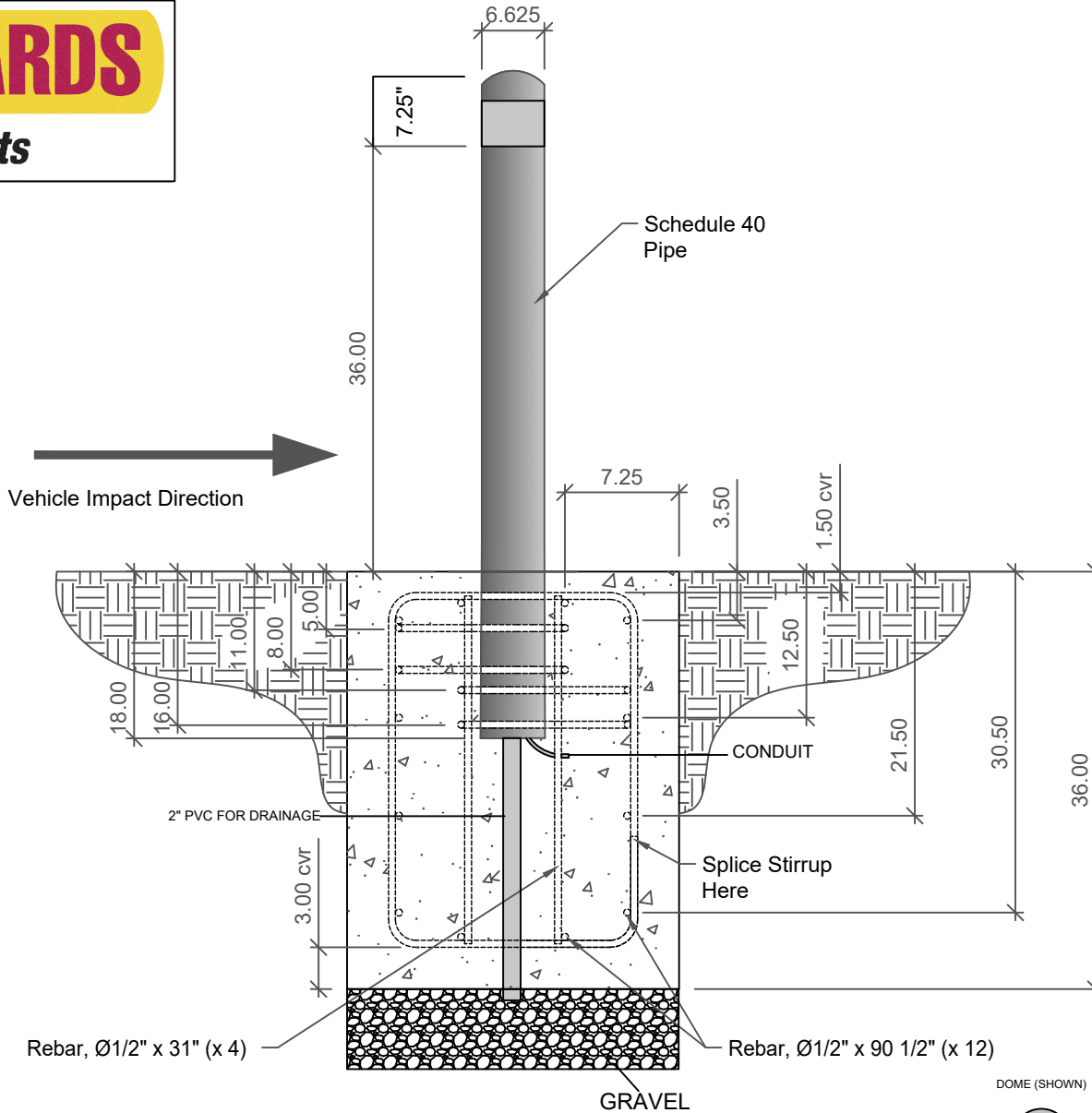
END VIEW-FOUNDATION
